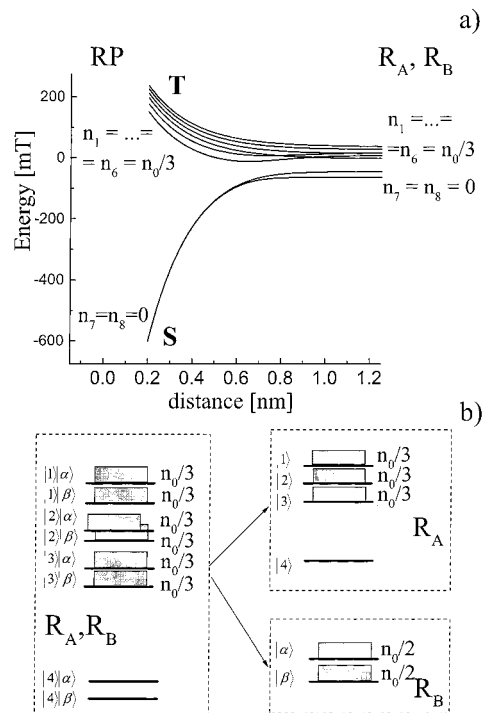
Figure 1. (a) Calculated scheme of the energy levels of RP with one magnetic nucleus as a function of interradical distance; J(r) = J_0 \exp(-(r-R)/\lambda) , J_0 = 400 mT, R = 0.2 nm, \lambda = 0.2 nm, a = 70 mT, and B_0 = 20 mT. (b) Correlation scheme for the RP- and radical-level populations.
